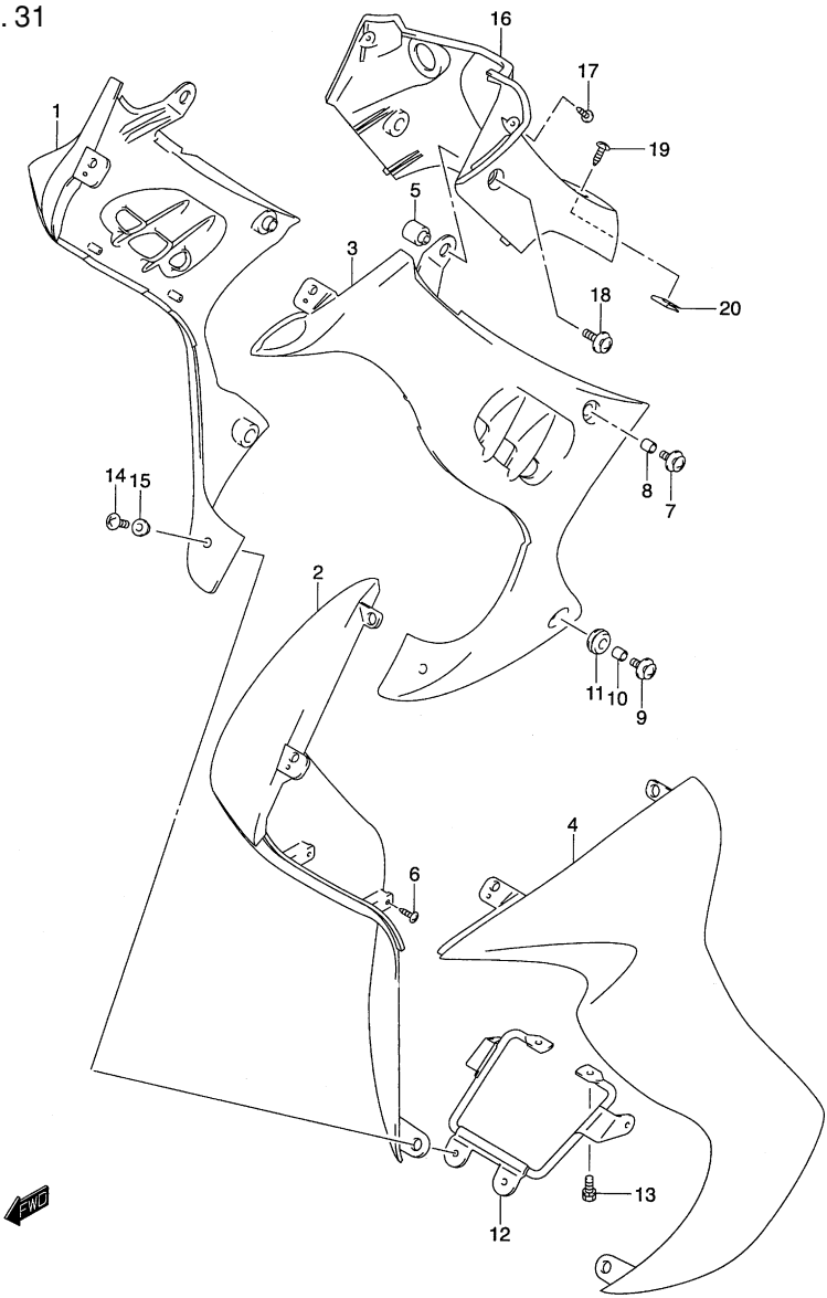
FIG.31 (E-11) LEG SHIELD
