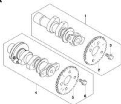
FIG.126A (1-B-11) CAMSHAFT/VALVE
