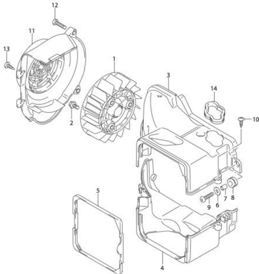
REF.NO. PART NO. DESCRIPTION QTY REMARKS 1 17110-09J00-000 FAN, COOLING 1 2 01550-0612A-000 BOLT 3 3 17121-09JB0-000 COWLING, CYLINDER UPPER 1 4 17122-09JA0-000 COWLING, CYLINDER LOWER 1 5 17123B09J00N000 MOLD, CYLINDER COWLING 1 6 09160-06129-000 WASHER (6.5X16X1) 1 7 09180-06307-000 SPACER (6.5X9X10) 1 8 09320-09016-000 CUSHION 1 9 02112B0625AN000 SCREW 1 10 03541-0516A-000 SCREW 2 11 17130-09J00-000 COWLING, FAN 1 12 02112-1625A-000 SCREW 2 13 03541-0516A-000 SCREW 2 14 17124-39J00-000 MOLD, TENSIONER ADJUSTER 1
