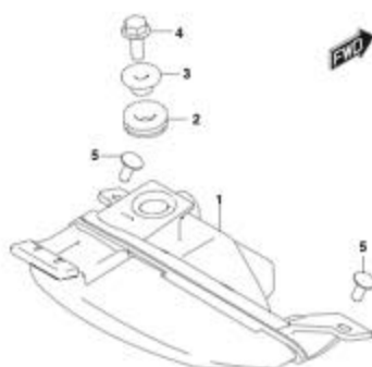
FIG.339A (1-D-9) REAR COMBINATION LAMP
