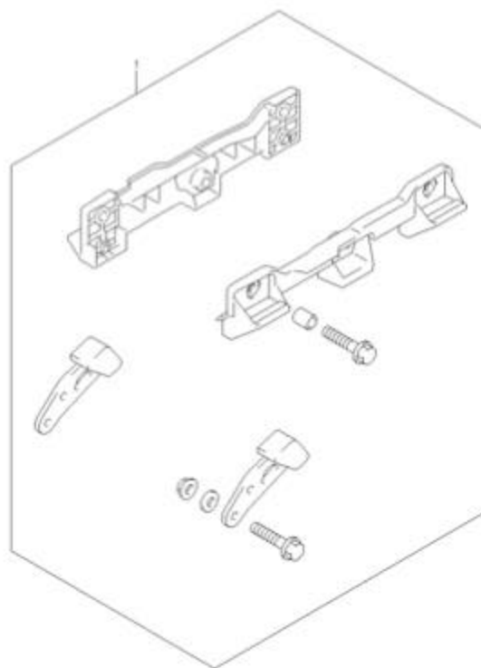
DL1000AL4_E99_976 SIDE CASE BRACKET SET (OPTIONAL)
