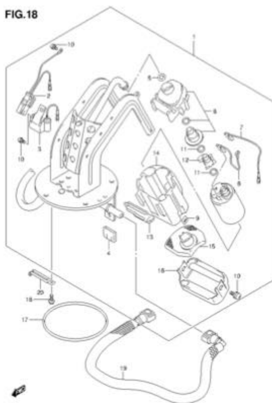
FIG.18 (1-C-7) FUEL PUMP
