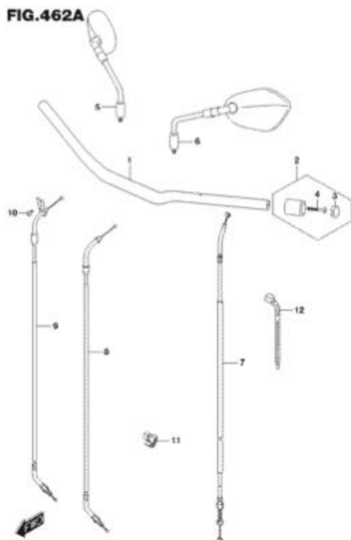
FIG.462A (1-F-6) HANDLEBAR
