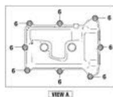
FIG.102A (1-B-3) CYLINDER HEAD COVER
