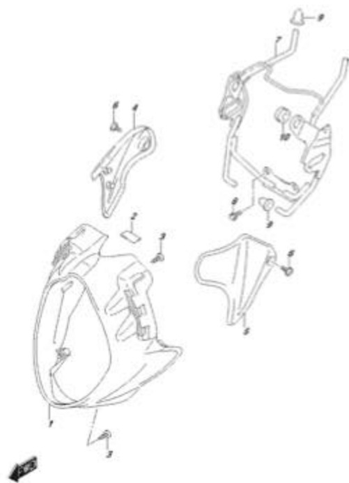
SFV650AL5_E99_452A HEADLAMP COVER
